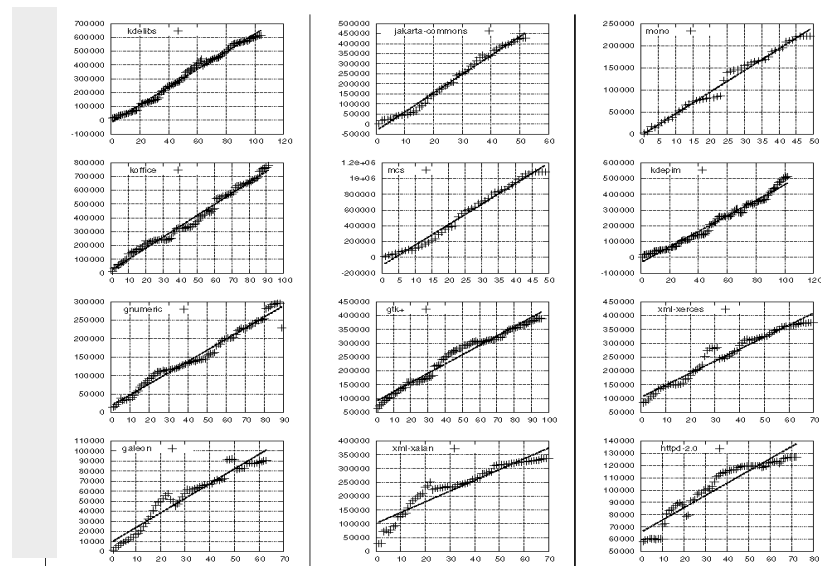
Linear growth of large projects' file sizes during months following version 1 release : 12 of 18 libre source projects Source: Robles et al (2005)
